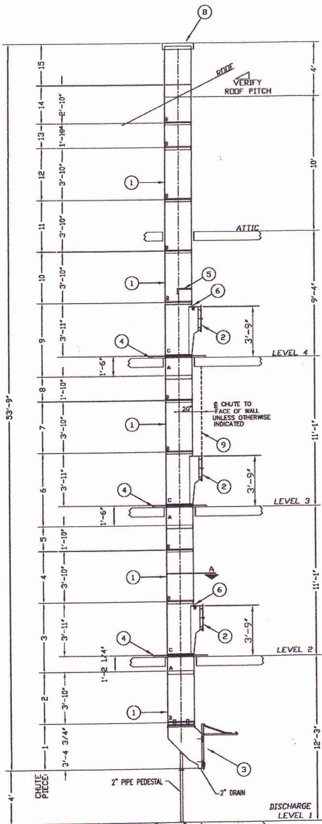
CHUTE ELEVATION VIEW ONE 24" DIAMETER LINEN CHUTE (3) THREE INTAKE DOORS
